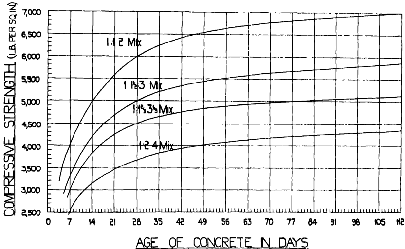
Fig. 329.—Effect of Age on Strength of Concrete.
